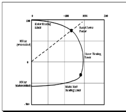
Figure 3: Generator MVAR versus MW Capability
