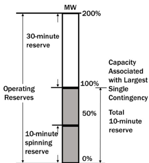
Figure 12: Operating Reserve Requirements
